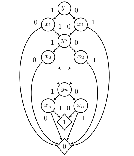
Figure 1 BDD for \bigwedge_{i=1}^n x_i \equiv y_i .
