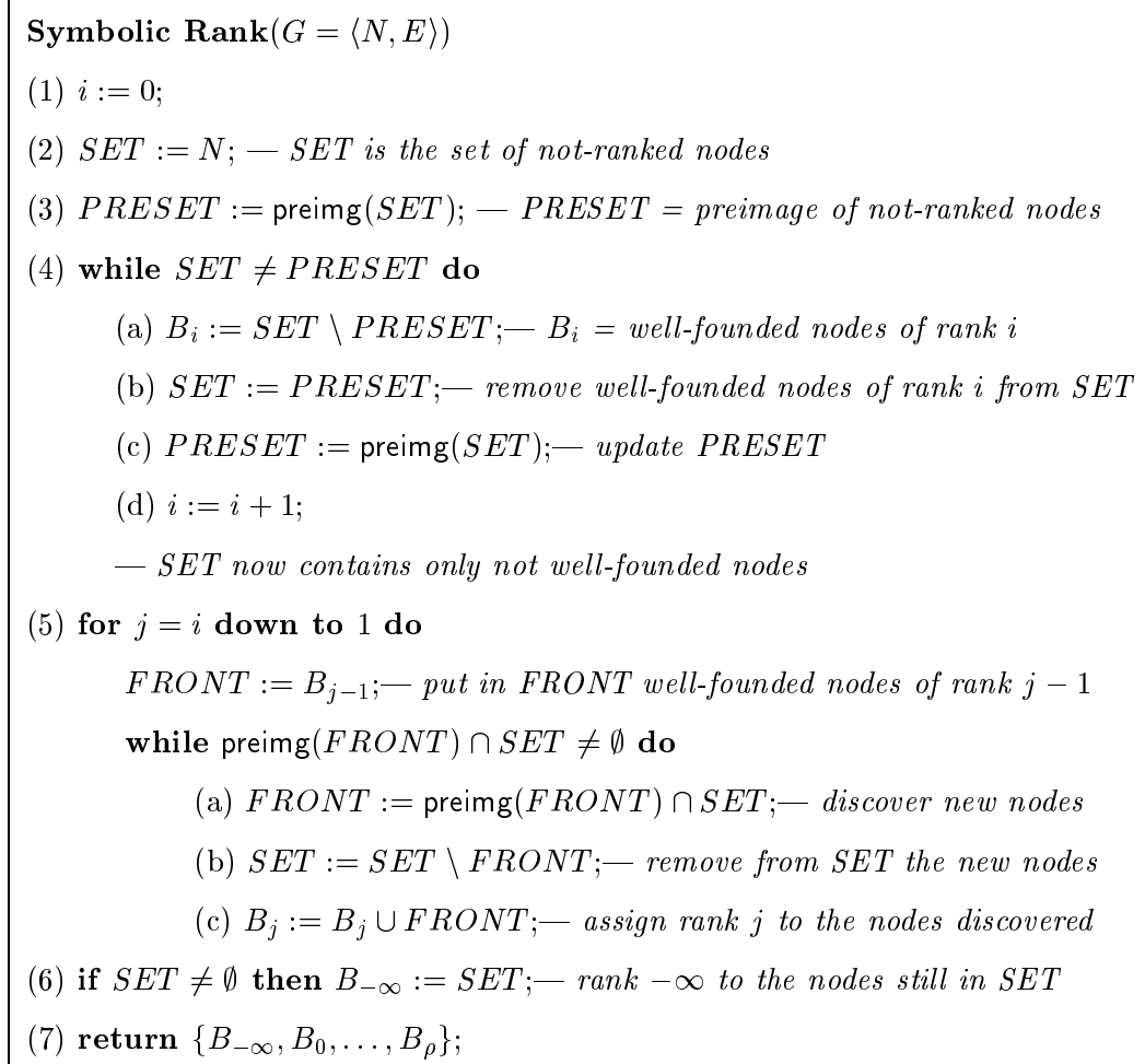
Fig. 2. The Symbolic Rank algorithm
