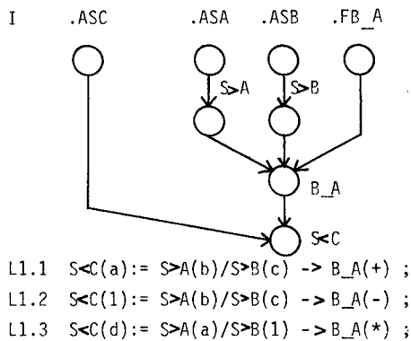
Figure 13 Limited Allocated Structure and Bound Space
