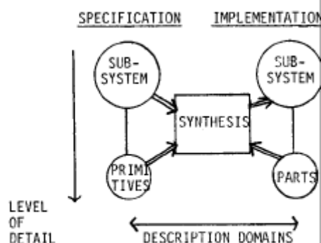
Figure 2 Synthesis Parameter Definition
