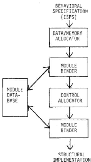
Figure 9 CMU-DA Synthesis Flow
